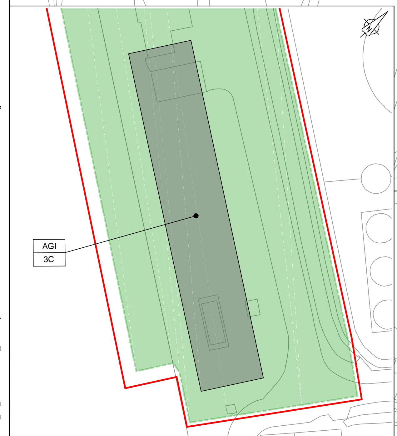
ENLARGED PLAN - AGI SCALE 1:500
